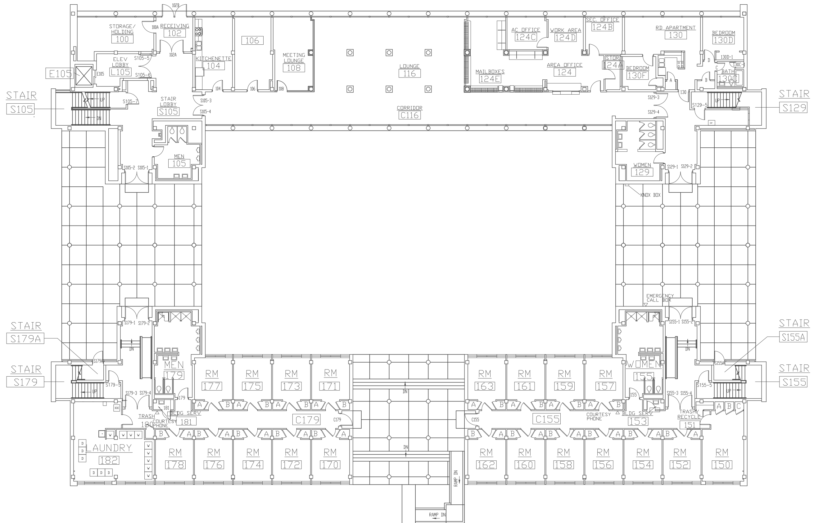
SNYDER HALL First Floor Plan
